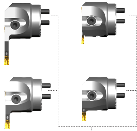
Serrated Modular Heads Chromium-Molybdenum Alloy Steel Hardened to 40-44 HRC Nickel-Plated Thru Coolant
